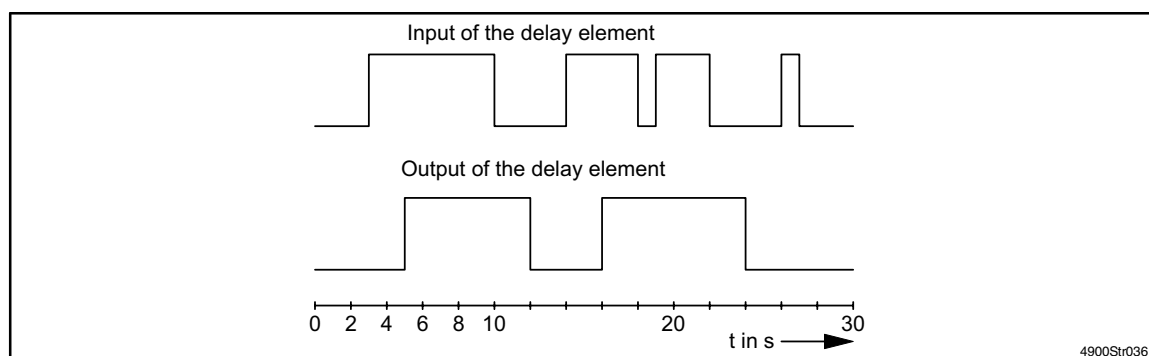
FIG 7-9 Signal flow for a delay time of 2s (C128 = 2s)
