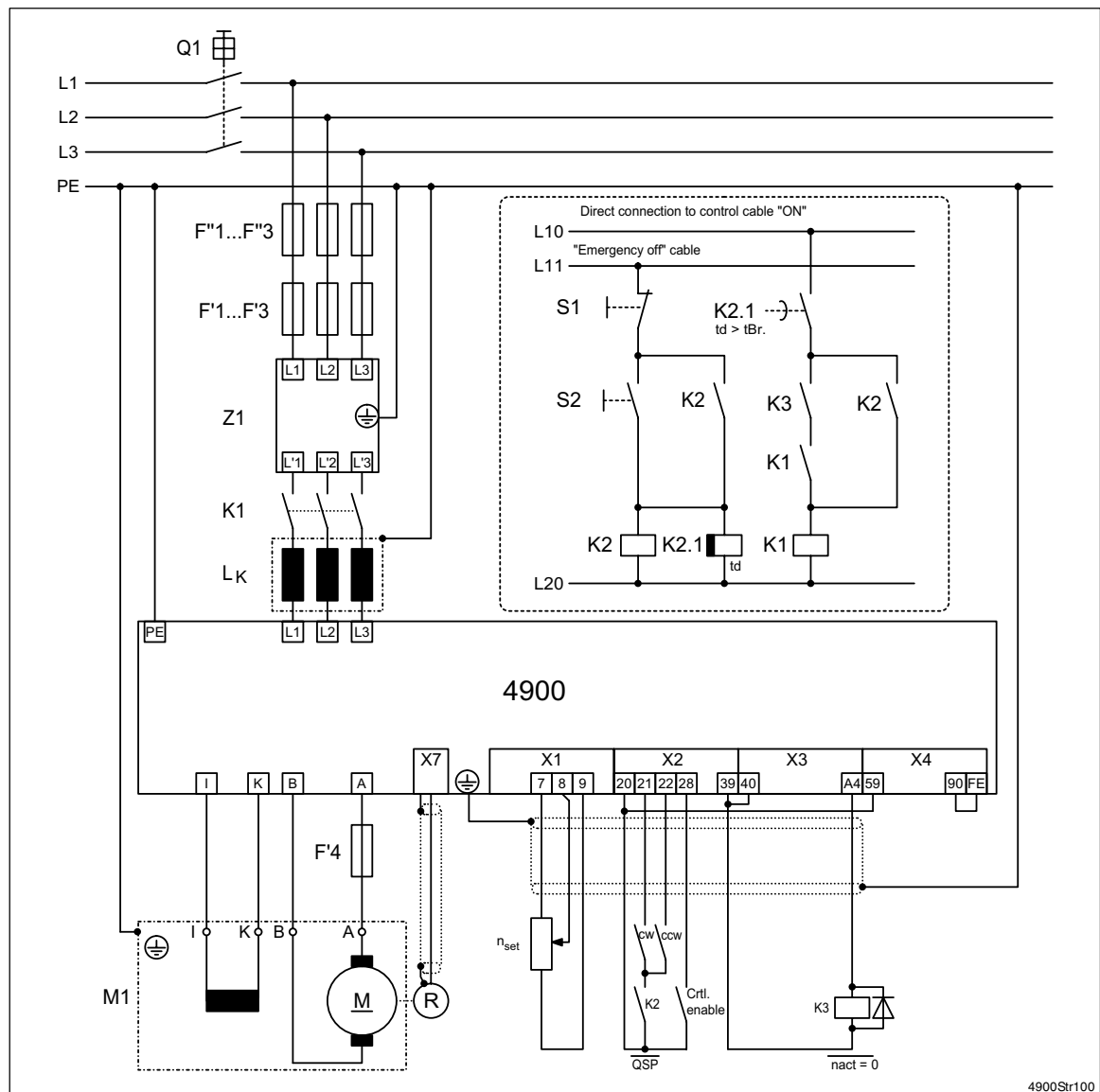
FIG 15-2 Connection diagram for speed control with resolver
