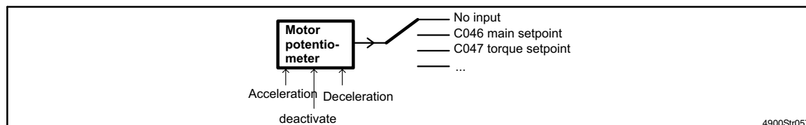
FIG 7-30 Motor potentiometer
