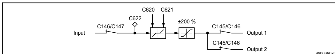
FIG 7-43 Dead-band element
