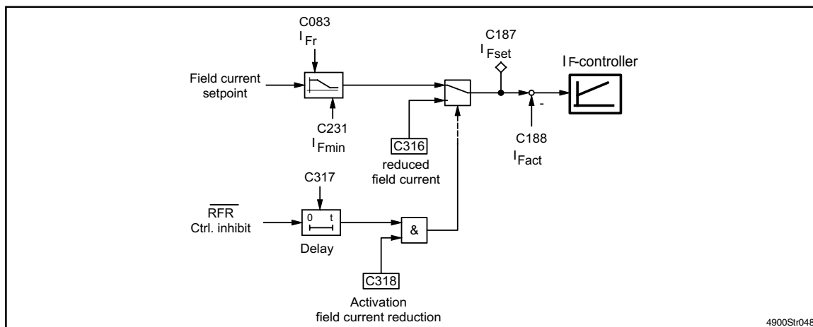
FIG 7-21 Standstill excitation
